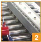
Side belt drive with belt over roller technology
